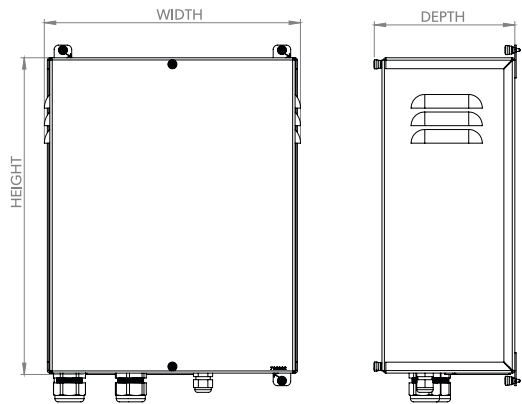
VARCX120 VFD ENCLOSURE
